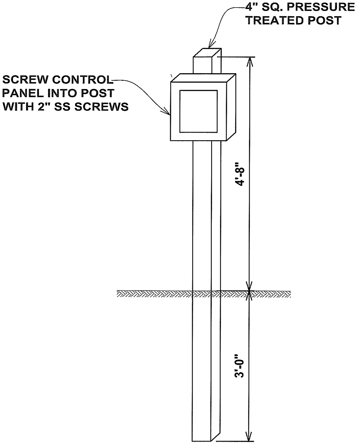
GRINDER PUMP MOUNTING DETAIL NOT TO SCALE
